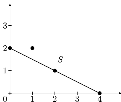
FIGURE 4. N_{\phi_i}^+(F) .
