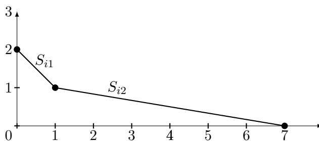
FIGURE 6. N_{\phi_i}^+(F) .
