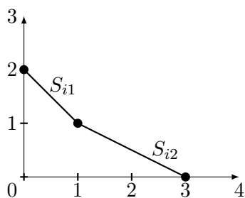
FIGURE 5. N_{\phi_i}^+(F) .
