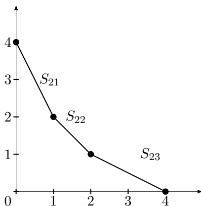
FIGURE 3. N_{\phi_2}^+(F) .
